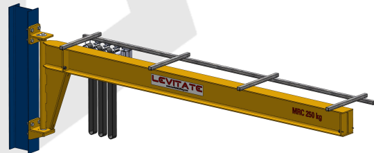
Wall Mounted Under Braced Jib Crane
